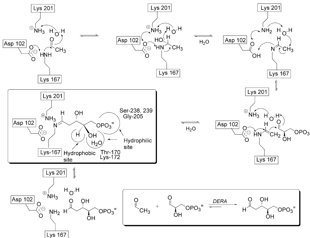
Figure 1. Mechanism of DERA catalyzed aldol reaction between the natural donor acetaldehyde and acceptor D-glyceraldehyde-3-phosphate to generate D-2-deoxyribose-5-phosphate. The reaction proceeds through a Schiff base intermediate. The proton shuffling system composed of Asp102 and Lys201, a key water molecule to mediate proton transfer, 6 another key water involved in enantioselective acceptor binding and the residues interacting with the acceptor substrate side chains are shown.
