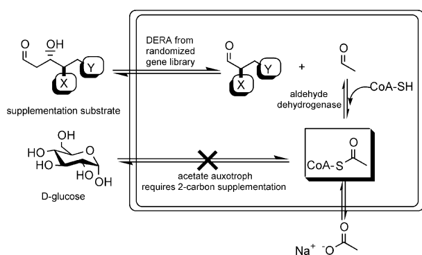
Figure 6. The metabolically engineered SELECT ( \Delta ace , \Delta adhC , DE3 ) E. coli strain requires 2-carbon supplementation for cell growth. In the absence of acetate supplementation, only those cells transformed with a DERA gene variant can catalyze the retro-aldol reaction of the supplementation substrate and survive. Thus, any enzyme selectivity that releases acetaldehyde or acetate may be selected.
