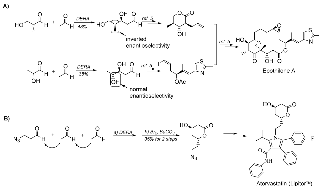
Figure 5. DERA catalyzed synthesis of designed substrates.
