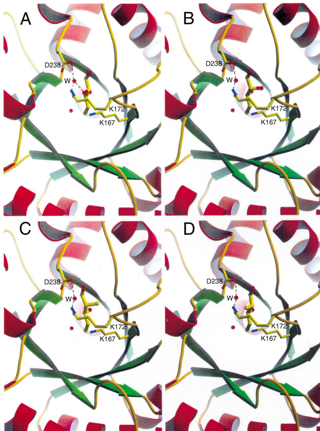
Figure 4. DERA product modeling based on the Schiff base complex structure (PDB code 1JCJ). 6 The enzyme model contains the S238D mutation. Four product molecules were modeled into the active site and the energy of the complex minimized. The enzyme is able to catalyze the aldol reaction with D-glyceraldehyde and D-2-methyl-3-hydroxy propanol resulting in the products displayed in A and C, respectively (Figs 1 and 5). The structures shown in B and D resulting from the corresponding enantiomeric acceptors are not substrates for DERA.
