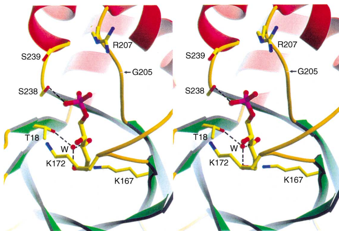
Figure 3. Stereoview of the active site of the DERA carbinolamine complex. The central beta barrel is depicted by the \beta -strand colored in green. Upon reaction of the substrate D-2-deoxyribose-5-phosphate with the reactive lysine, Lys167, the carbinolamine is formed. Thr18 is hydrogen bonded via a water molecule to the substrate. Also Ser238 forms a hydrogen bond with the phosphate group of the substrate. Residues shown in the figure, which are mutated in the present study are K172E, G205E, R207E, S238D and S239E. A water molecule is shown to have H-bonding interaction with K172, T18 and the C4-OH group of the substrate.
