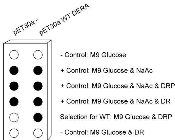
Figure 7. Proof of concept for the selection protocol using SELECT . SELECT cells require a 2-carbon source for growth. Neither DR nor DRP is toxic to the cells. The cells transformed with the empty vector (–) do not grow in the presence of DRP but the WT DERA expressing cells do. Neither transformant grows when supplemented only with DR for which DERA has a 53,000-fold poorer specificity constant compared to DPR. Both transformants grow when the medium is supplemented with sodium acetate (NaAc).
