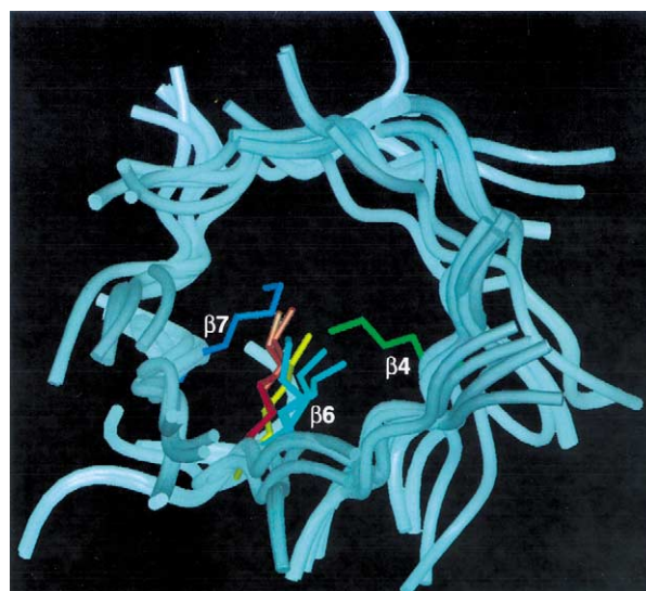
Figure 2. Overlap of eight known aldolase \alpha/\beta barrels showing the Lys residue for Schiff base formation. DERA Lys167 is depicted in yellow.
